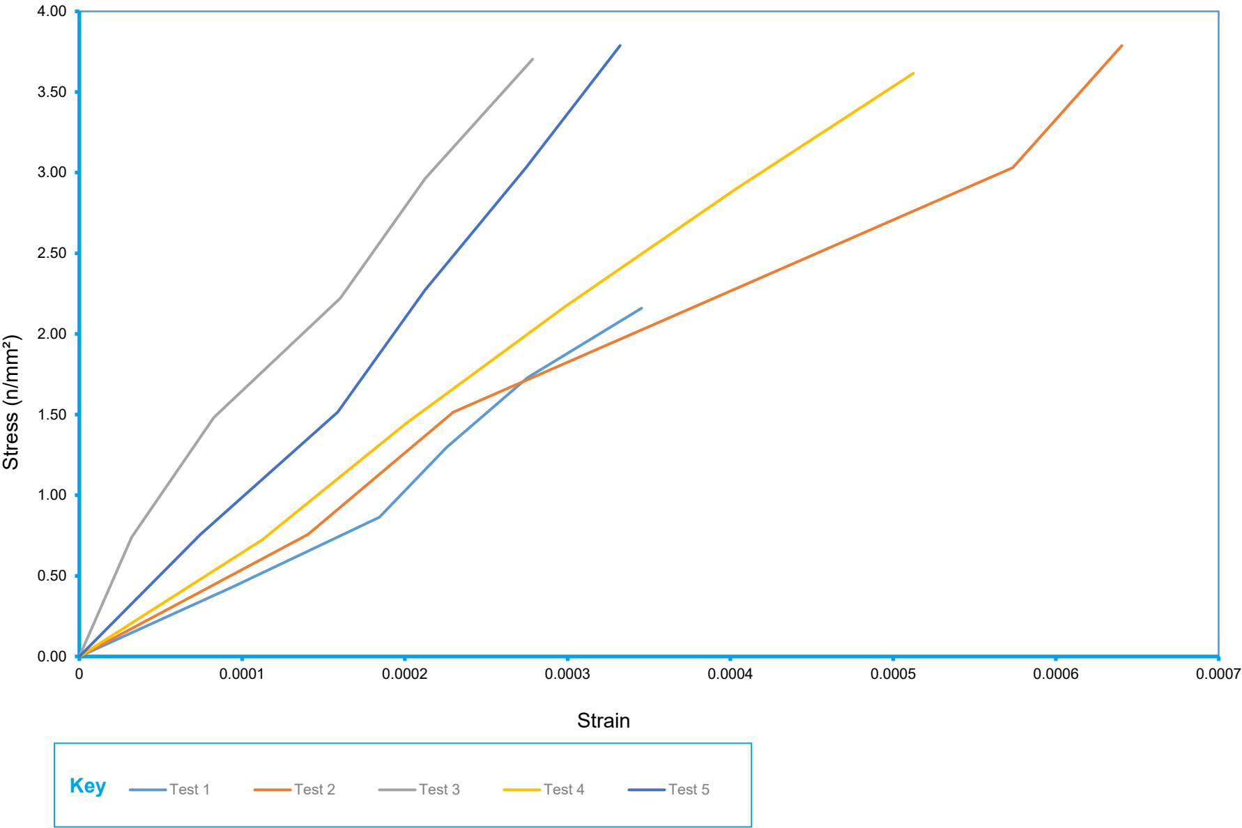
Chart 1 - Stress vs Strain for Specimens Tested Under Compressive Load to BS EN 1052-1:1999
